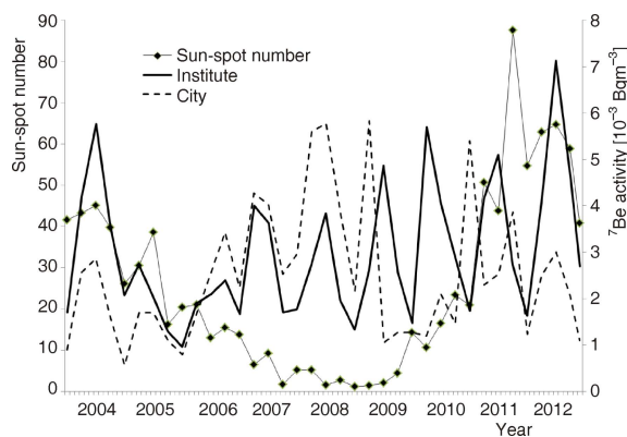
Figure 5. Seasonal activities of ^7\text{Be} and seasonal sun-spot numbers
