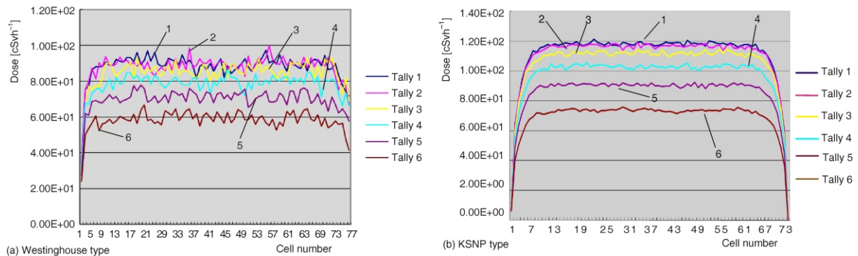
Figure 4. Evaluation results for the neutron dose [ \text{cSv h}^{-1} ]
