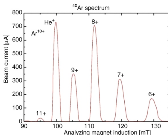
Figure 7. Spectrum of argon ions optimized for maximal production of Ar 8+ ions
