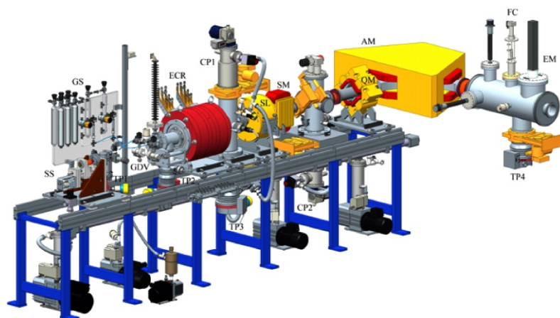
Figure 6. The refurbished subsystems of the ECR ion source; GS – gas inlet system, SS – solid substance inlet system, GDV – gas dosing valves, TP1, TP2, TP3, TP4 – turbomolecular pumps, CP1, CP2 – cryogenic pumps, ECR – ion source body, SL – solenoid lens, SM – steering magnet, QM – quadrupole magnet, AM – analyzing magnet, FC – Faraday cup, and EM – emittance meter
