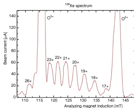
Figure 8. Spectrum of xenon ions optimized for maximal production of Xe 23+ ions
